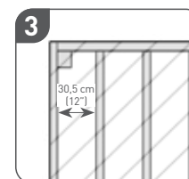
30,5 cm (12") DIAGONAL INSTALLATION SUBSTRUCTURE 30,5 cm (12") on center maximum joists. More severe angles may require closer joist spacing
