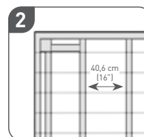
40,6 cm (16") PICTURE FRAME INSTALLATION SUBSTRUCTURE 40,6 cm (16") on center maximum joists plus additional support for picture frame structure (30,5 cm (12") on center for commercial applications)
