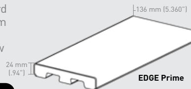
TimberTech EDGE Collection (3- Sided Cap)
