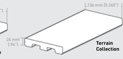
TimberTech PRO Collection (4- Sided Cap)
